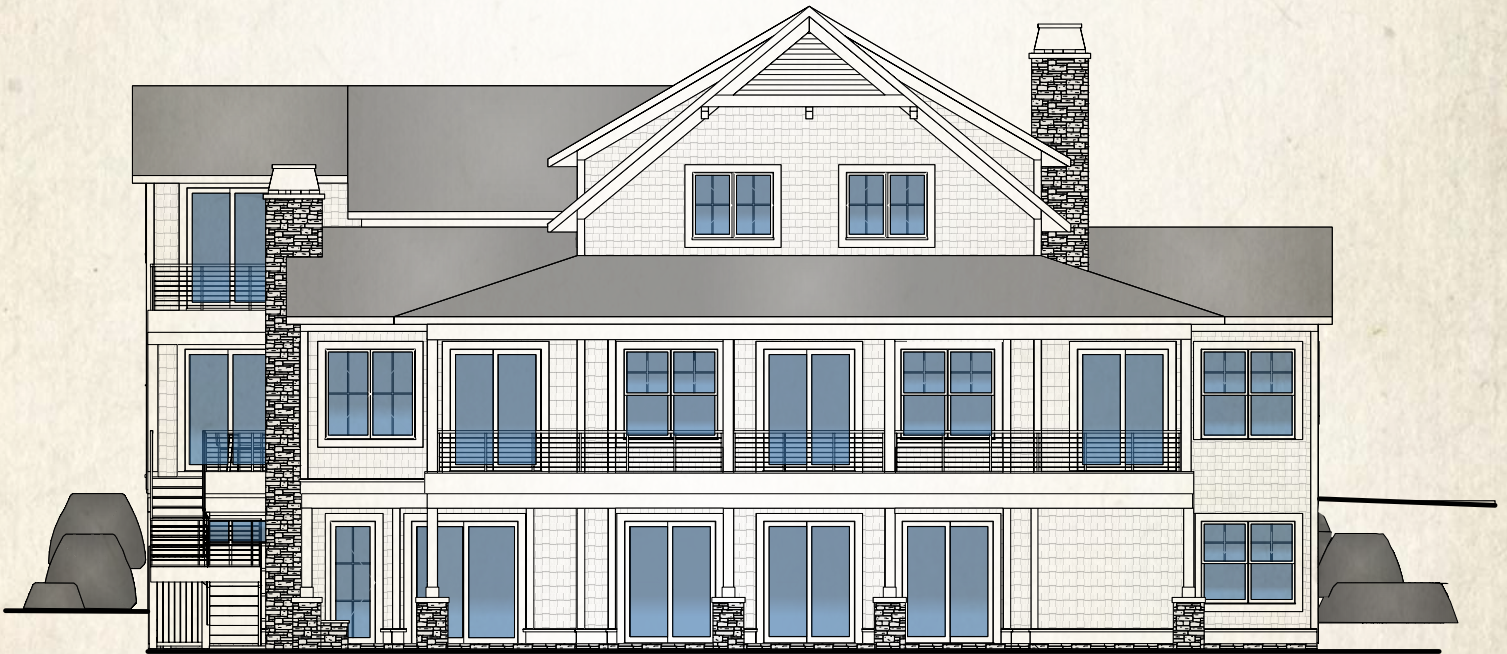
West Elevation
